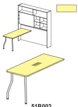
51B002 1500x616x731
